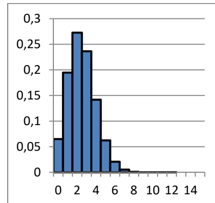
n = 15. B(15, 1/6).
